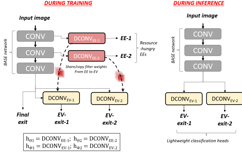
Figure 6: Depiction of QUTE during training and inference. The early-exits (EE) are only used during training for weight-transfer. During inference, the EEs are removed, and only EV-exits are retained. We do not include other layers such as dense and pointwise convolution in the figure for brevity.
