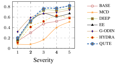
(c) AUPRC TinyImagenet-C
