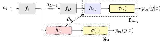
Figure 2: Early-view-assistance architecture. One assisting early-exit g_{\theta_k} and corresponding early-view-assisted exit f_{out_k} is shown. Early-exits weights \theta_k are transferred/copied to h_{\phi_k} before each train batch, i.e., \phi_k = \theta_k
