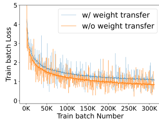
Figure 5: Batch-loss at EV-0 for CIFAR10 on Resnet-8
