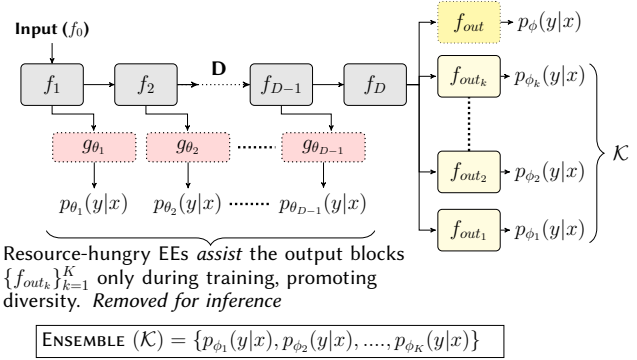
Figure 1: QUTE architecture. \{f_{out_k}\}_{k=1}^K represents the 'K' additional output blocks at the final exit, which are assisted by 'K' early-exit blocks \{g_{\theta_k}\}_{k=1}^K only during training to promote diversity (see Figure 2). For inference, all ( early-exits & f_{out} ) are removed
